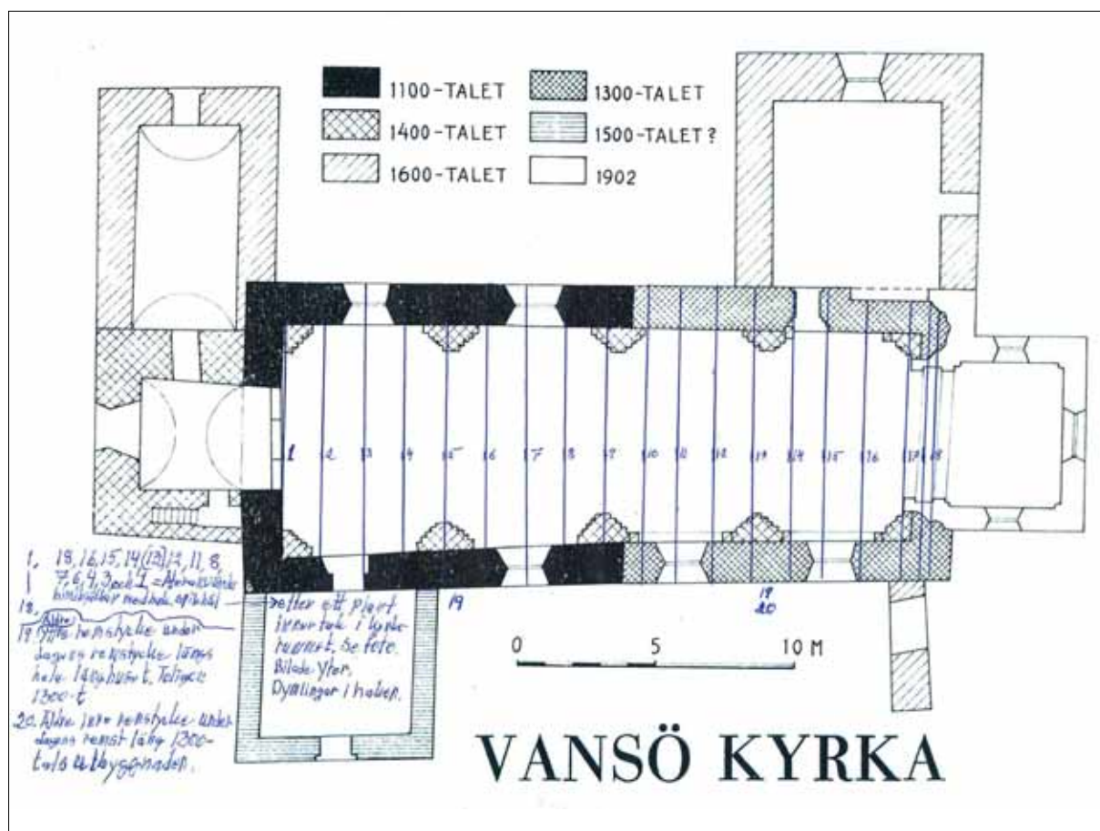
213 Planritning.
