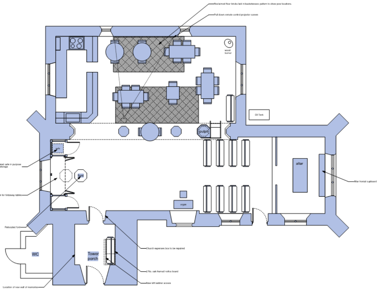
Plan 1:50 Proposed plan
