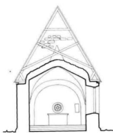
SKÄRNING C-C.
